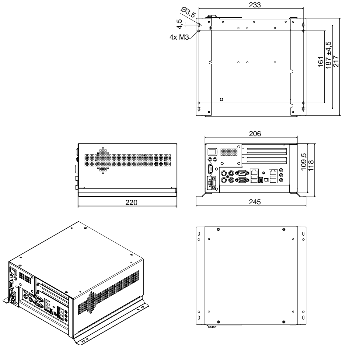
Floor mounting of the P400MA
